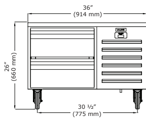
Front (36" Model)
