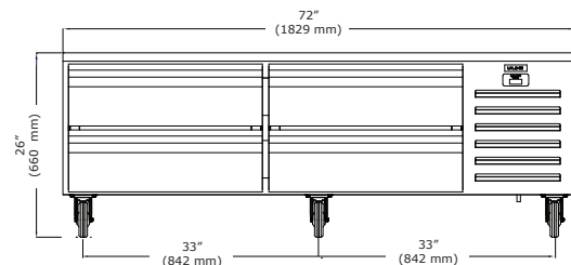
Front (72" Model)
