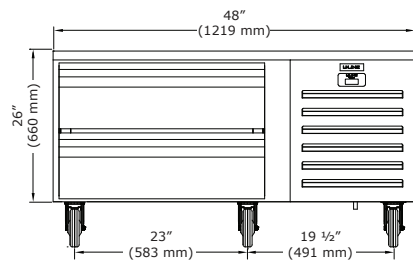
Front (48" Model)
